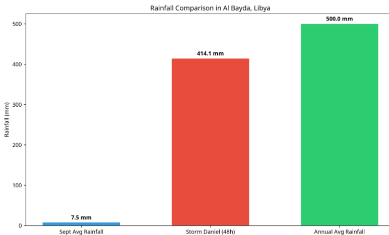
Figure 3: Comparison of rainfall in Al Bayda, Libya, during Storm Daniel (48h) against its typical September average and annual average, highlighting the extreme precipitation event.
