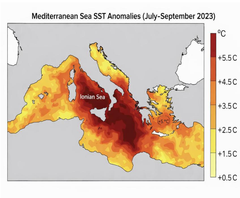
Figure 5: Heat map illustrating the significant positive Sea Surface Temperature anomalies across the Mediterranean Sea during the summer of 2023, with a notable +5.5°C anomaly in the Ionian Sea and North African coast region, contributing to Storm Daniel's intensification.
