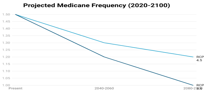
Figure 6: Multi-model projections showing stable or slightly declining Medicanes frequency under medium (RCP 4.5) and high (RCP 8.5) emission scenarios through the end of the 21st century.
