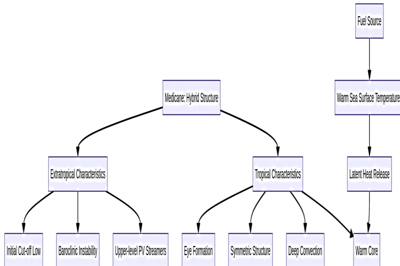
Figure 2: Conceptual diagram illustrating the hybrid nature of a Medican, combining tropical characteristics (warm core, deep convection) and extratropical characteristics (upper-level PV streamers, baroclinic instability).
