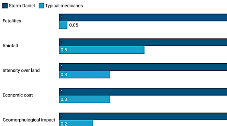
Figure 4: Comparison of Storm Daniel (2023) against typical historical Medicanes across five key impact dimensions. All values normalized to storm Daniel = 1.0. Data highlights the exceptional magnitude of Storm Daniel relative to previous events.
